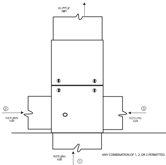
Figure 26 - Upflow Return Air Configurations and Restrictions
