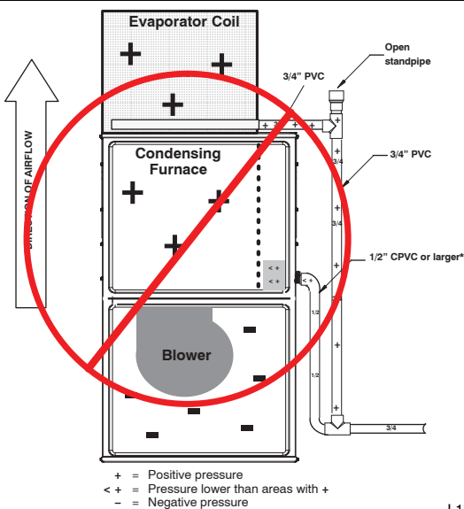
Figure 13 - Example of Field Drain Attachment (NOT ALLOWED)
