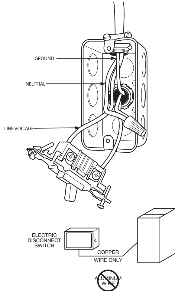
Figure 35 - Field-Supplied Electrical Box on Furnace Casing
