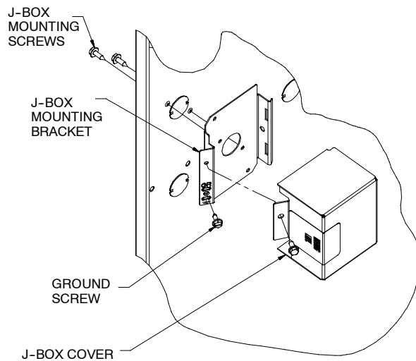
Figure 34 - Installing J-Box (When Used)
