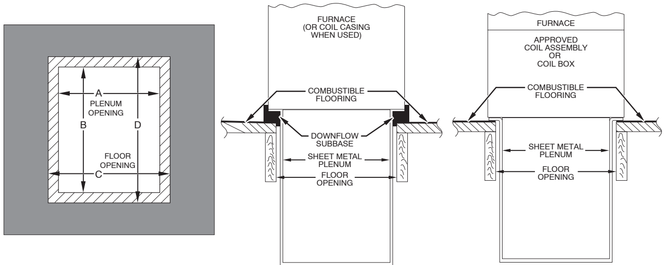
Figure 21 - Installation on Combustible Flooring
