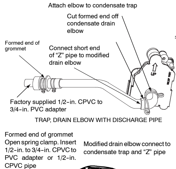
Figure 17 - Accessory Horizontal Drain Trap Grommet
