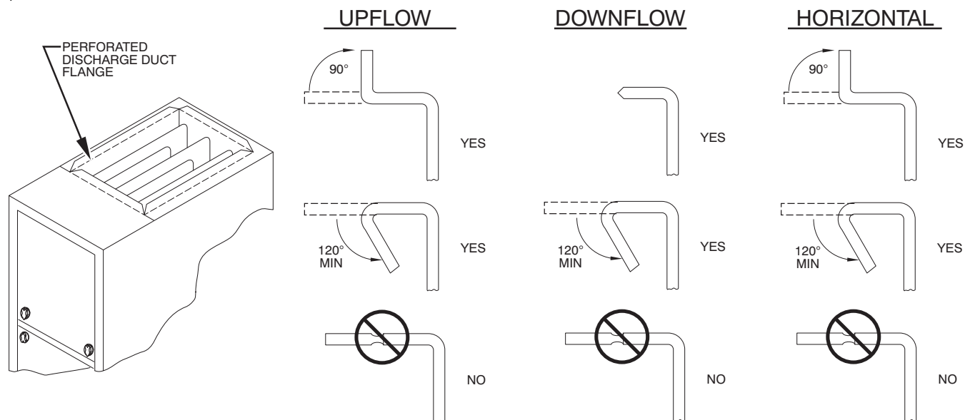
Figure 22 - Duct Flanges
