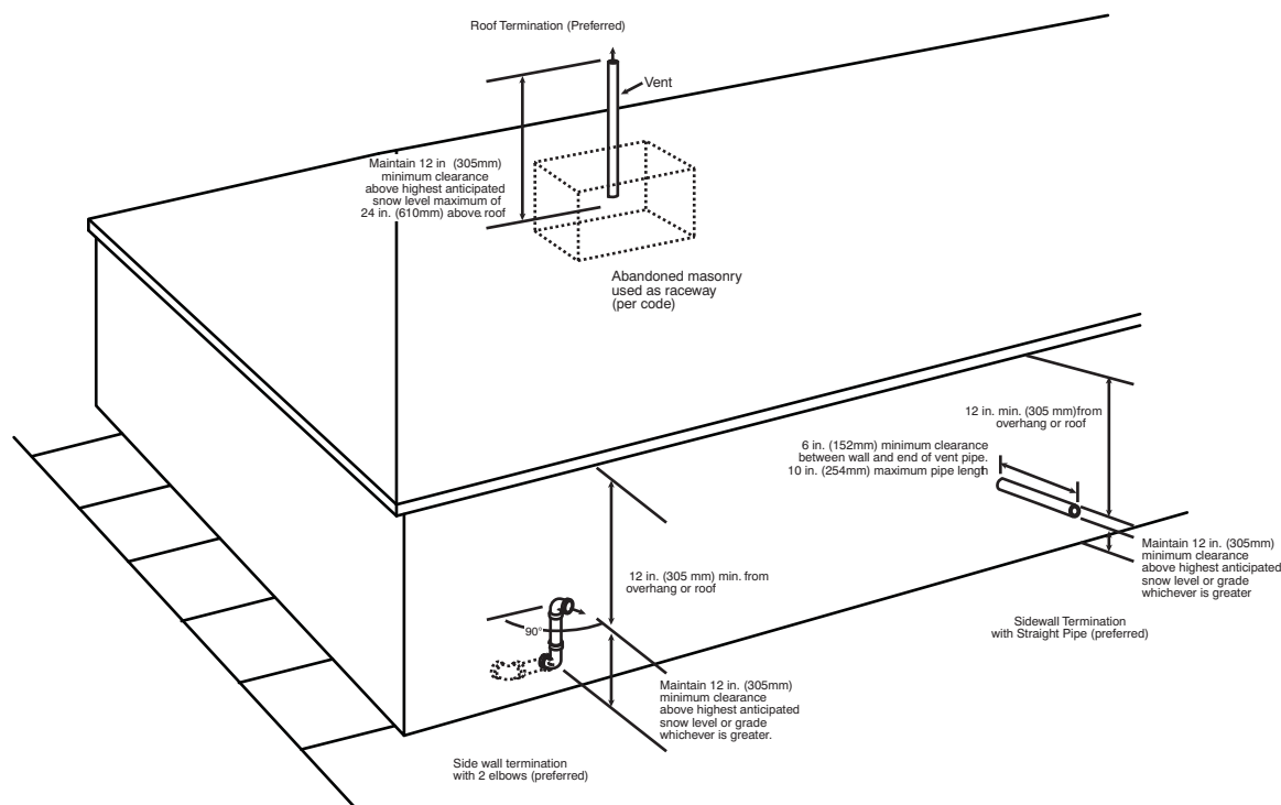
Figure 54 - Vent Pipe Termination for Non-Direct Vent and Ventilated Combustion Air System
