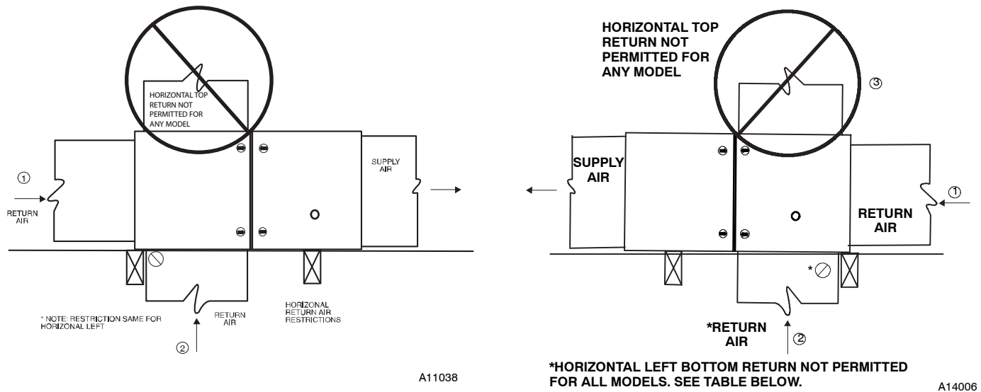
Figure 28 - Horizontal Return Air Configurations and Restrictions
