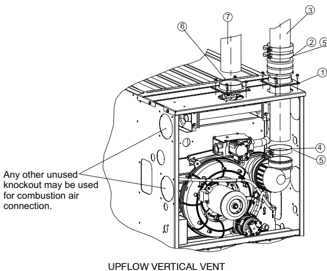
UPFLOW VERTICAL VENT
