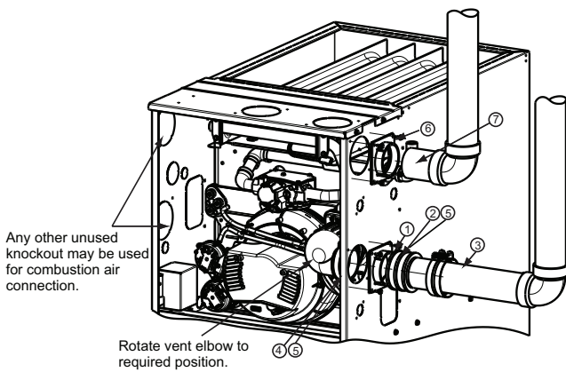
UPFLOW RIGHT CONFIGURATION
