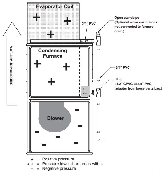
Example of Field Drain Attachment (continued)
