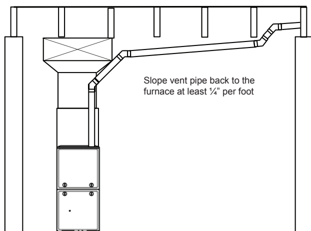
Figure 41 - Combustion-Air and Vent Pipe Diameter Transition Location and Elbow Configuration
