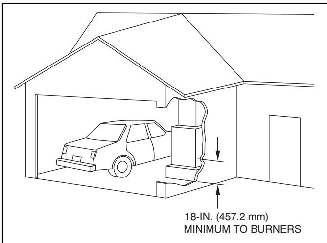
Figure 5 - Installation in a Garage
