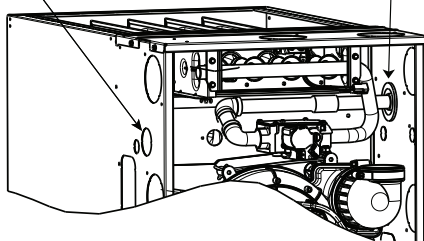
Figure 32 - Gas Entry
