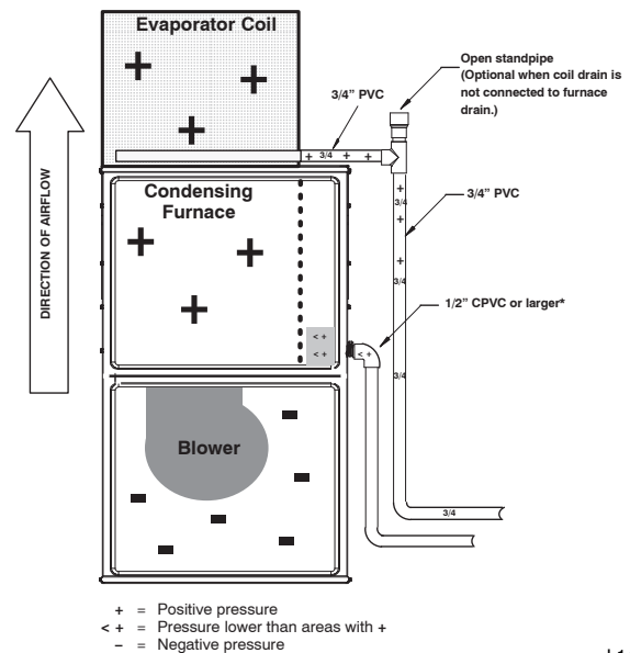
Figure 14 - Example of Field Drain Attachment
