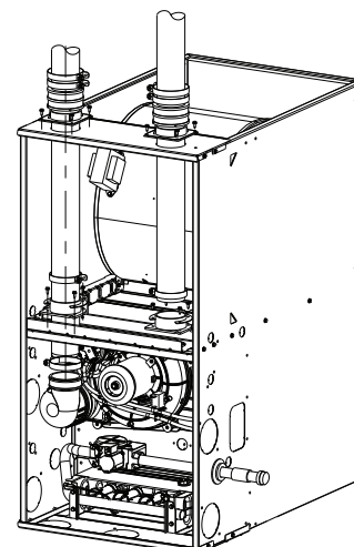
DOWNFLOW VERTICAL
