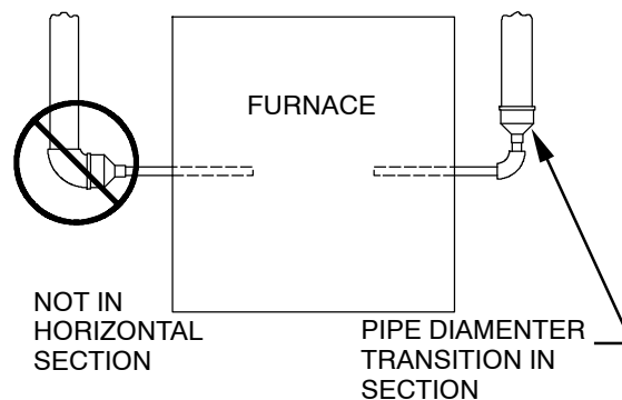
Figure 40 - Combustion-Air and Vent Pipe Diameter Transition Location and Elbow Configuration
