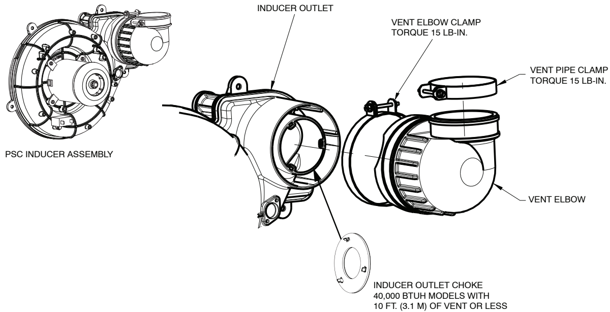
Figure 43 - Inducer Vent Elbow
