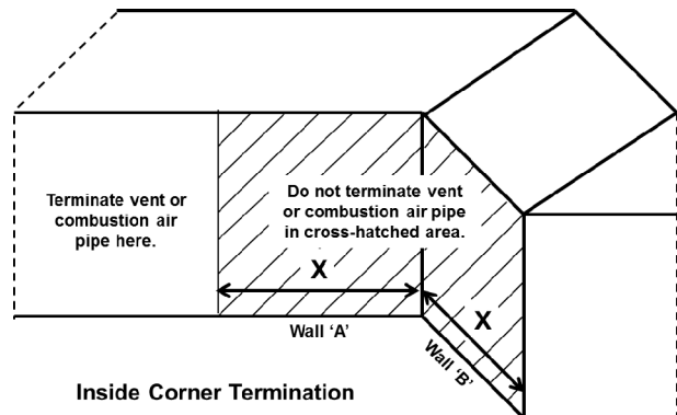
Figure 39 - Inside Corner Termination
