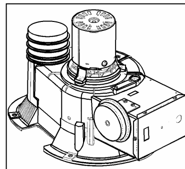
Train Blower Assembly AOS Part number 183505
